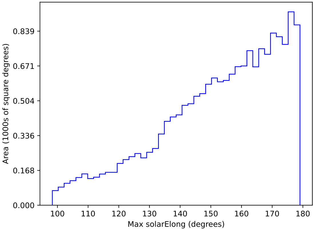
too_elab_r256_d2_gz_v3.4_10yrs WFD g band: Max solarElong
