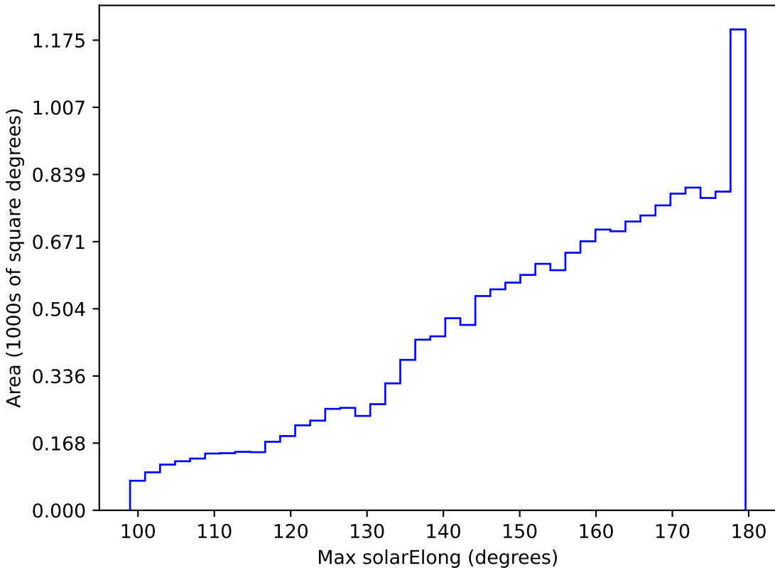
too_elab_r256_d2_gz_v3.4_10yrs WFD all bands: Max solarElong
