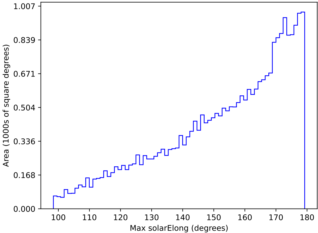
too_elab_r256_d2_gz_v3.4_10yrs All sky z band: Max solarElong
