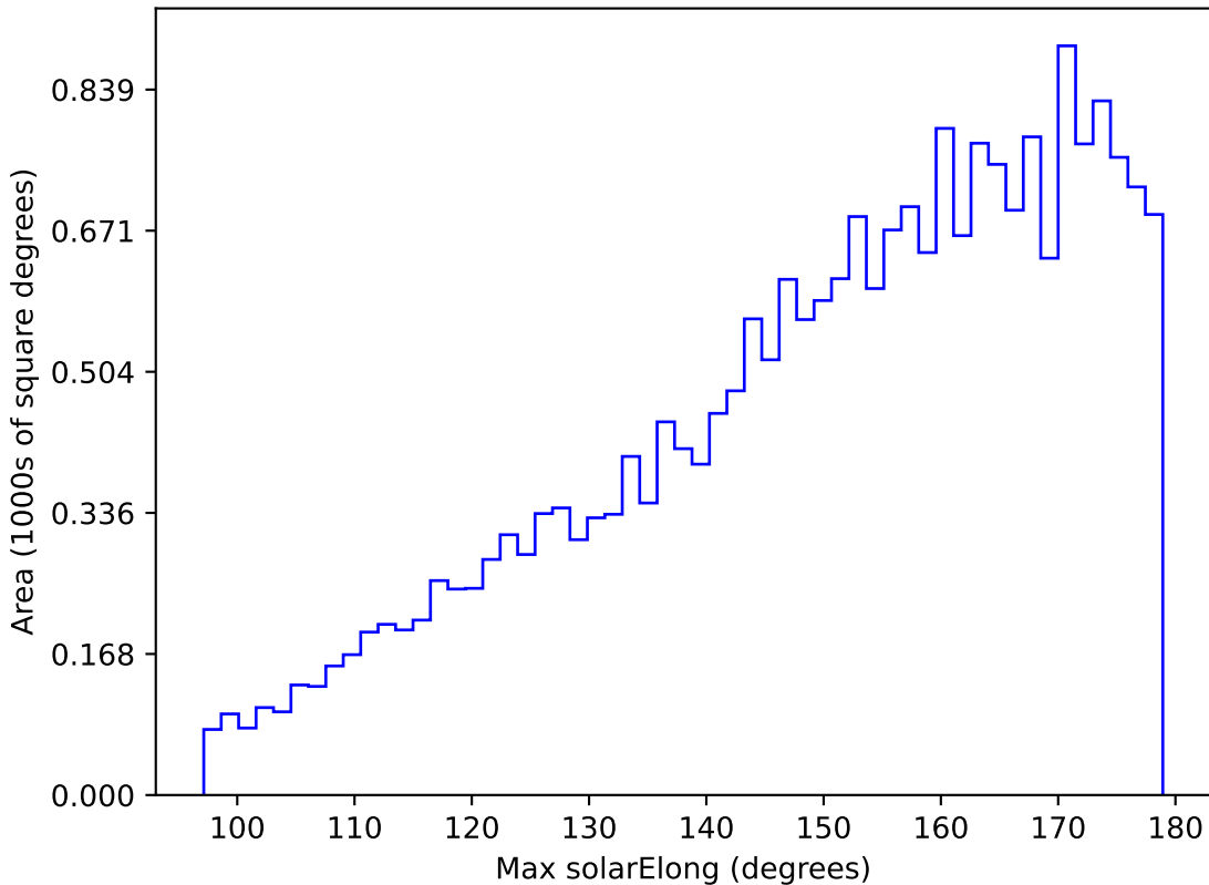
too_elab_r256_d2_gz_v3.4_10yrs All sky u band: Max solarElong
