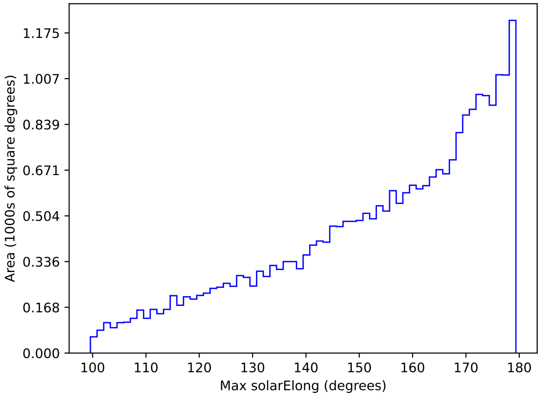
too_elab_r256_d2_gz_v3.4_10yrs All sky i band: Max solarElong
