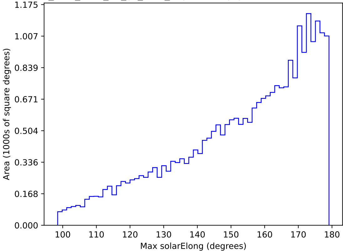
too_elab_r256_d2_gz_v3.4_10yrs All sky g band: Max solarElong
