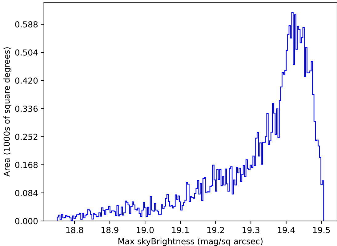
too_elab_r256_d2_gz_v3.4_10yrs Yr 1 z band: Max skyBrightness
