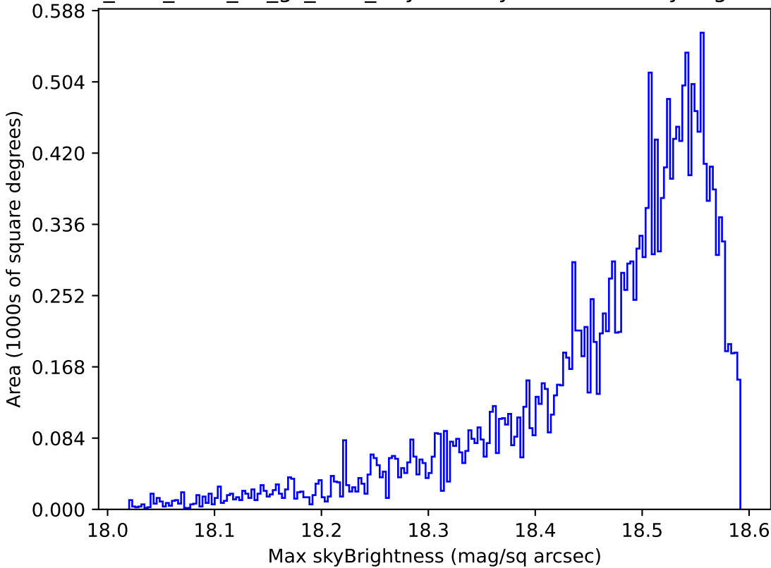
too_elab_r256_d2_gz_v3.4_10yrs Yr 1 y band: Max skyBrightness
