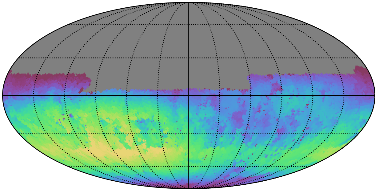
too_elab_r256_d2_gz_v3.4_10yrs Yr 1 u band: Max skyBrightness
