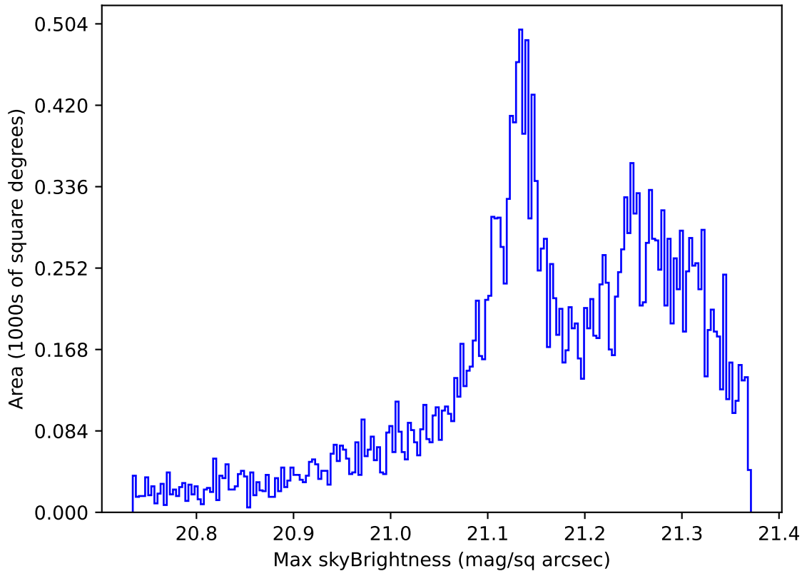
too_elab_r256_d2_gz_v3.4_10yrs Yr 1 r band: Max skyBrightness
