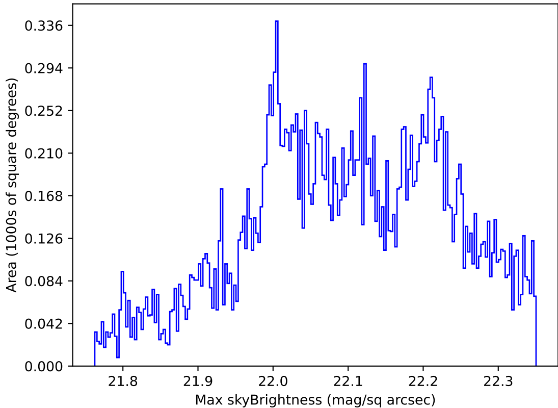
too_elab_r256_d2_gz_v3.4_10yrs Yr 1 g band: Max skyBrightness
