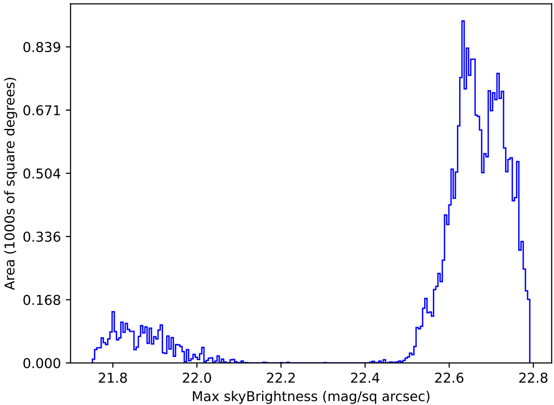
too_elab_r256_d2_gz_v3.4_10yrs Yr 1 all bands: Max skyBrightness
