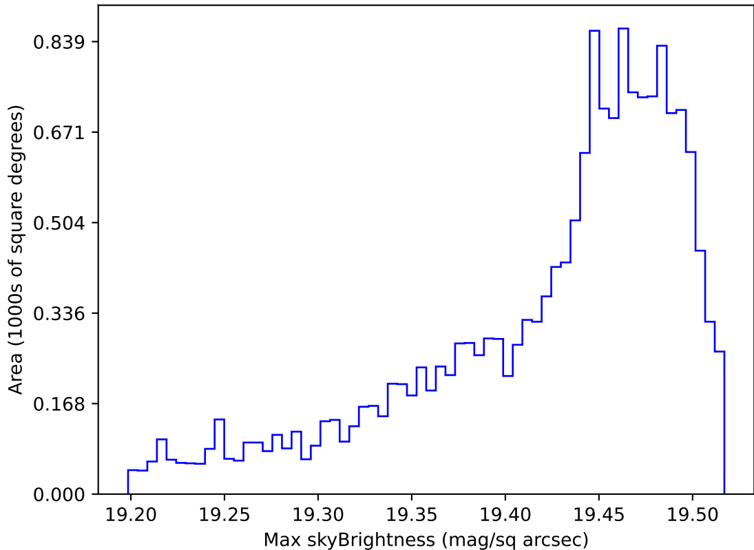
too_elab_r256_d2_gz_v3.4_10yrs WFD z band: Max skyBrightness
