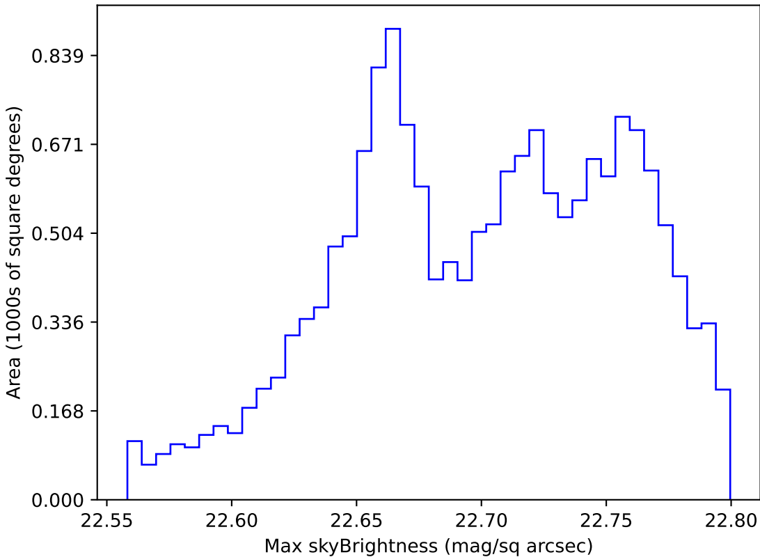
too_elab_r256_d2_gz_v3.4_10yrs WFD u band: Max skyBrightness
