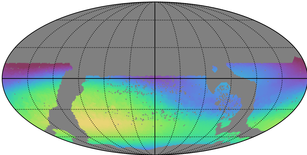
too_elab_r256_d2_gz_v3.4_10yrs WFD r band: Max skyBrightness
