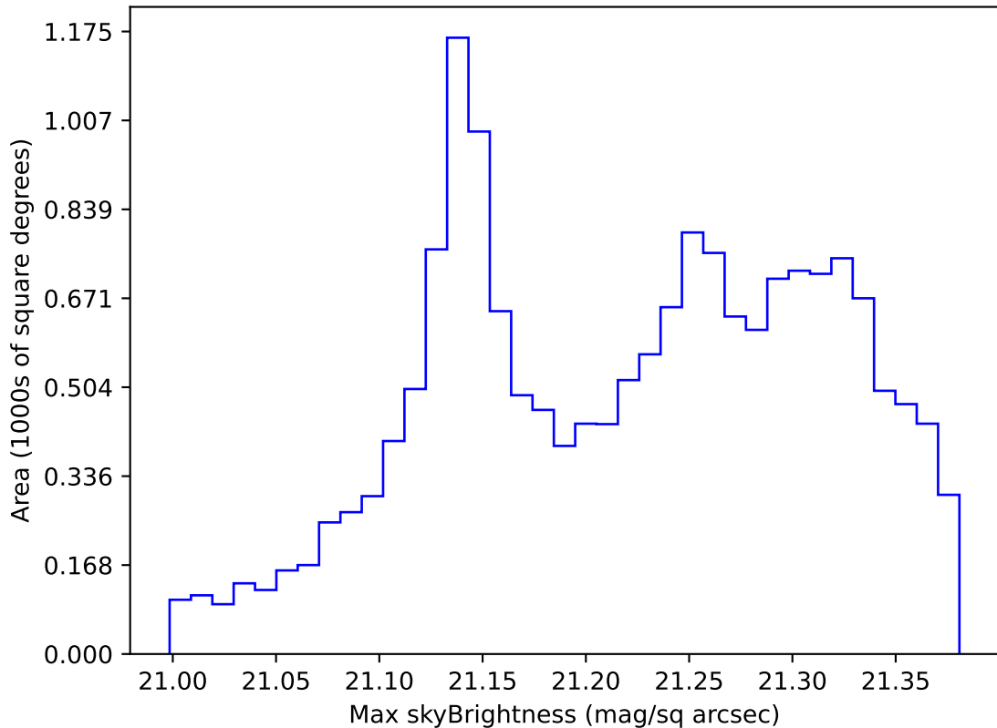
too_elab_r256_d2_gz_v3.4_10yrs WFD r band: Max skyBrightness
