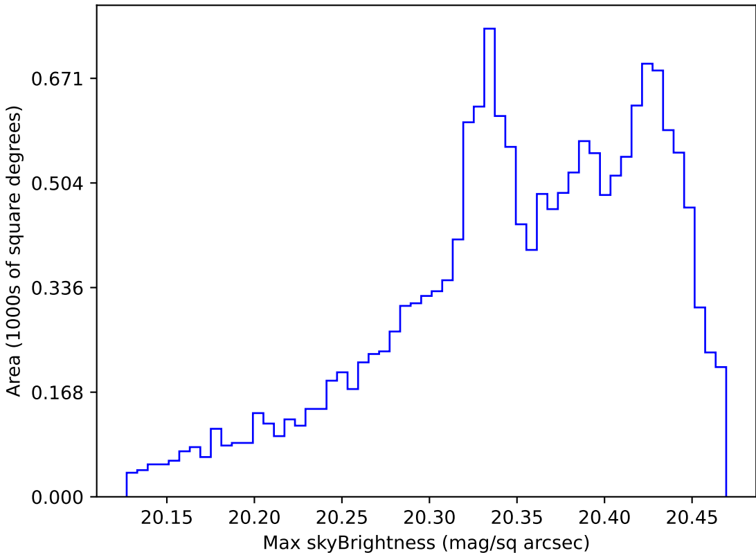
too_elab_r256_d2_gz_v3.4_10yrs WFD i band: Max skyBrightness
