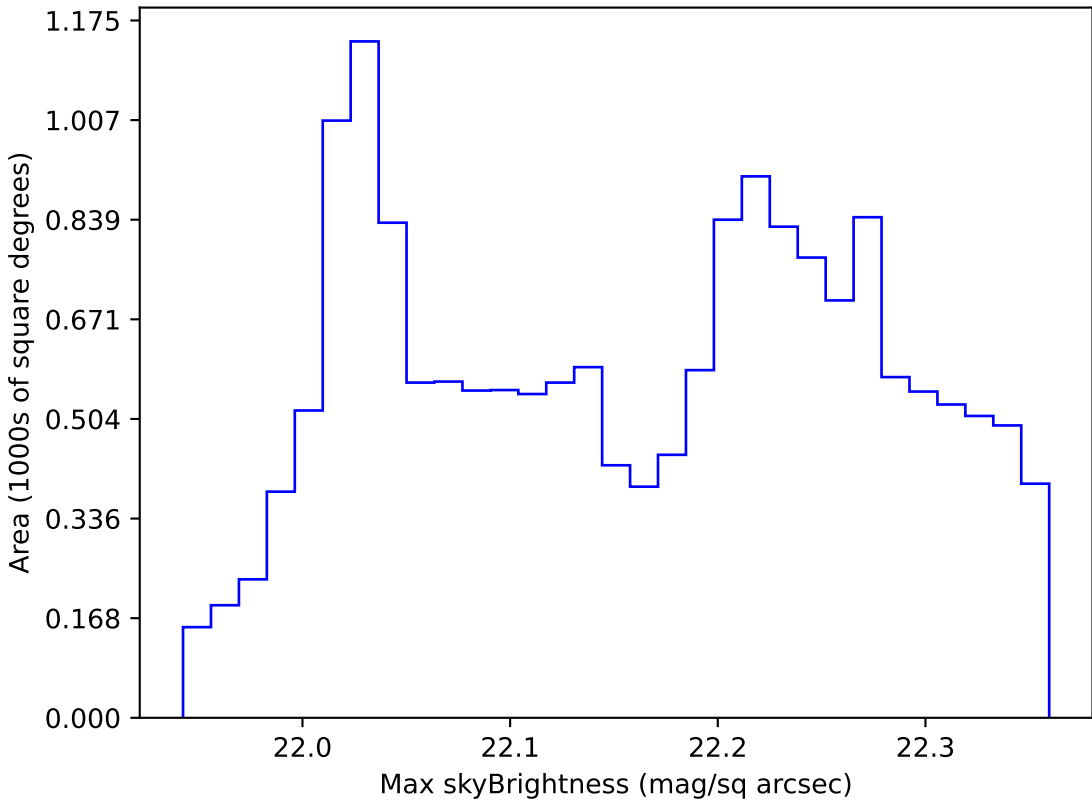
too_elab_r256_d2_gz_v3.4_10yrs WFD g band: Max skyBrightness
