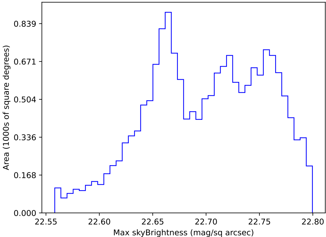
too_elab_r256_d2_gz_v3.4_10yrs WFD all bands: Max skyBrightness
