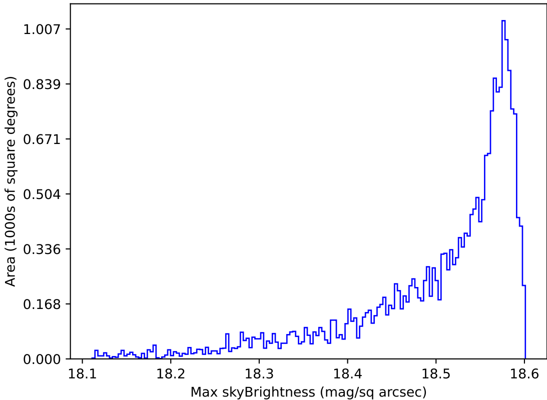
too_elab_r256_d2_gz_v3.4_10yrs All sky y band: Max skyBrightness
