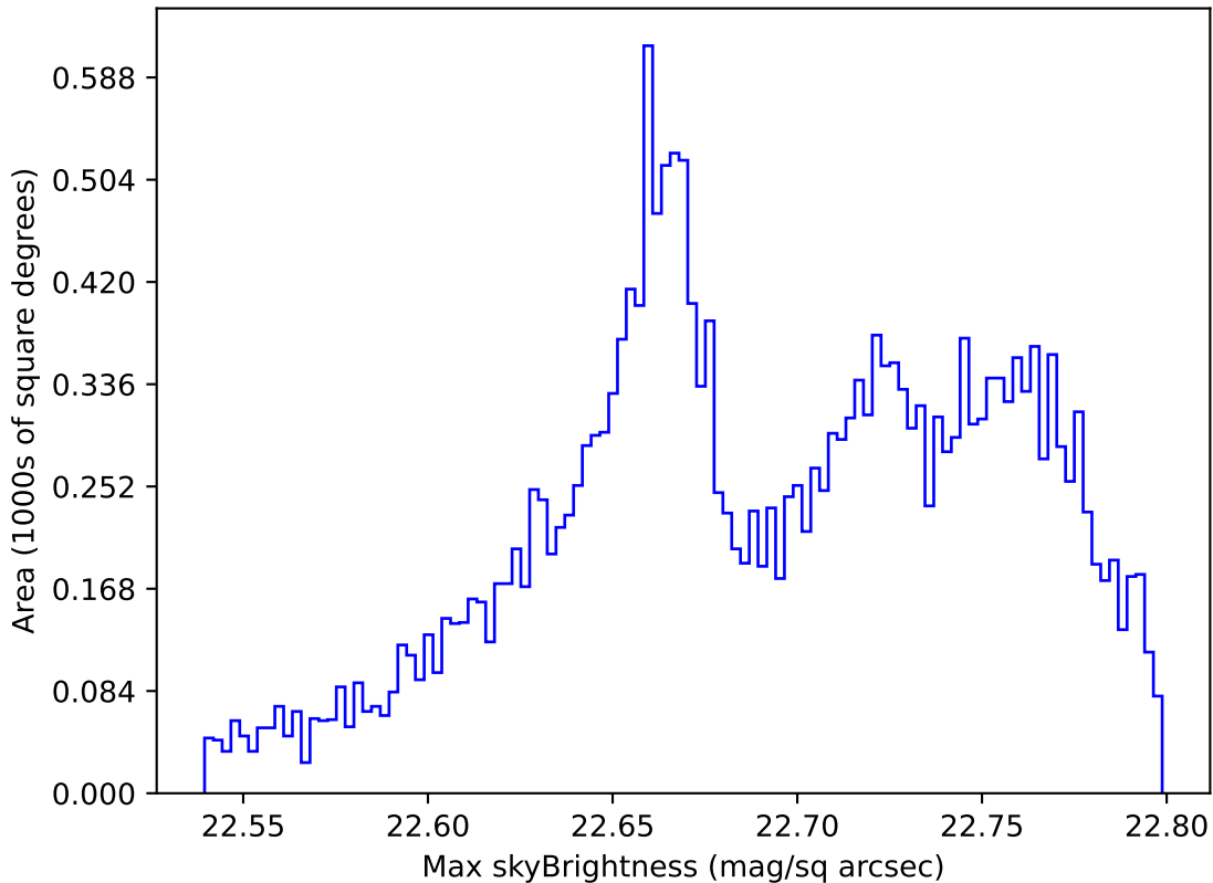
too_elab_r256_d2_gz_v3.4_10yrs All sky u band: Max skyBrightness
