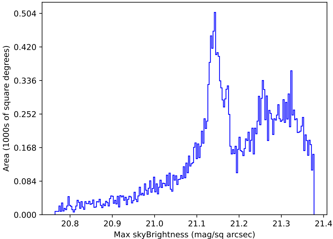
too_elab_r256_d2_gz_v3.4_10yrs All sky r band: Max skyBrightness
