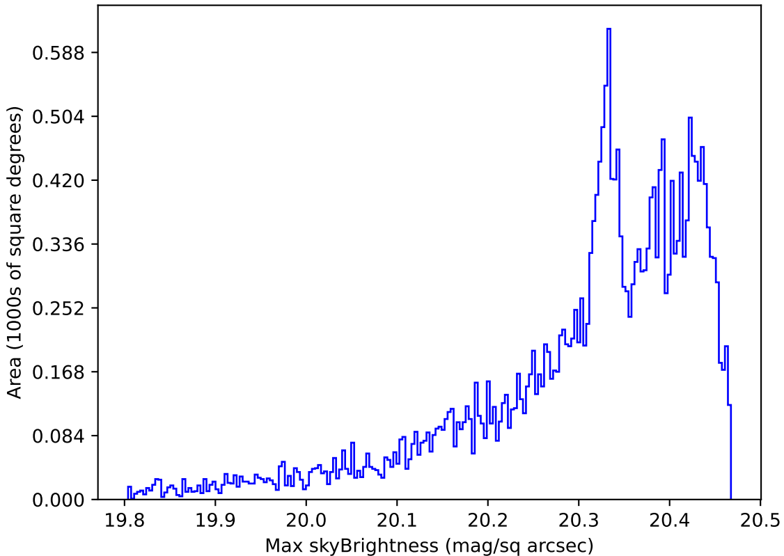
too_elab_r256_d2_gz_v3.4_10yrs All sky i band: Max skyBrightness
