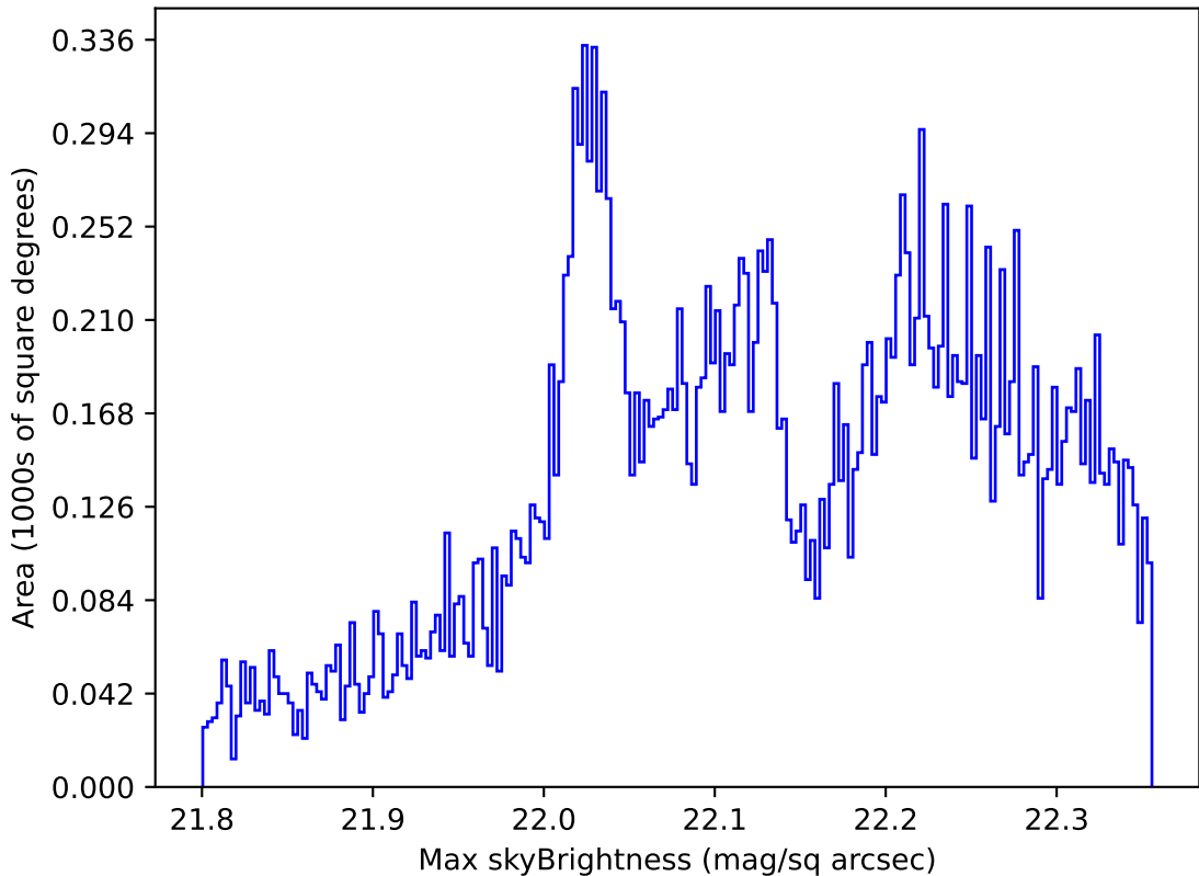
too_elab_r256_d2_gz_v3.4_10yrs All sky g band: Max skyBrightness
