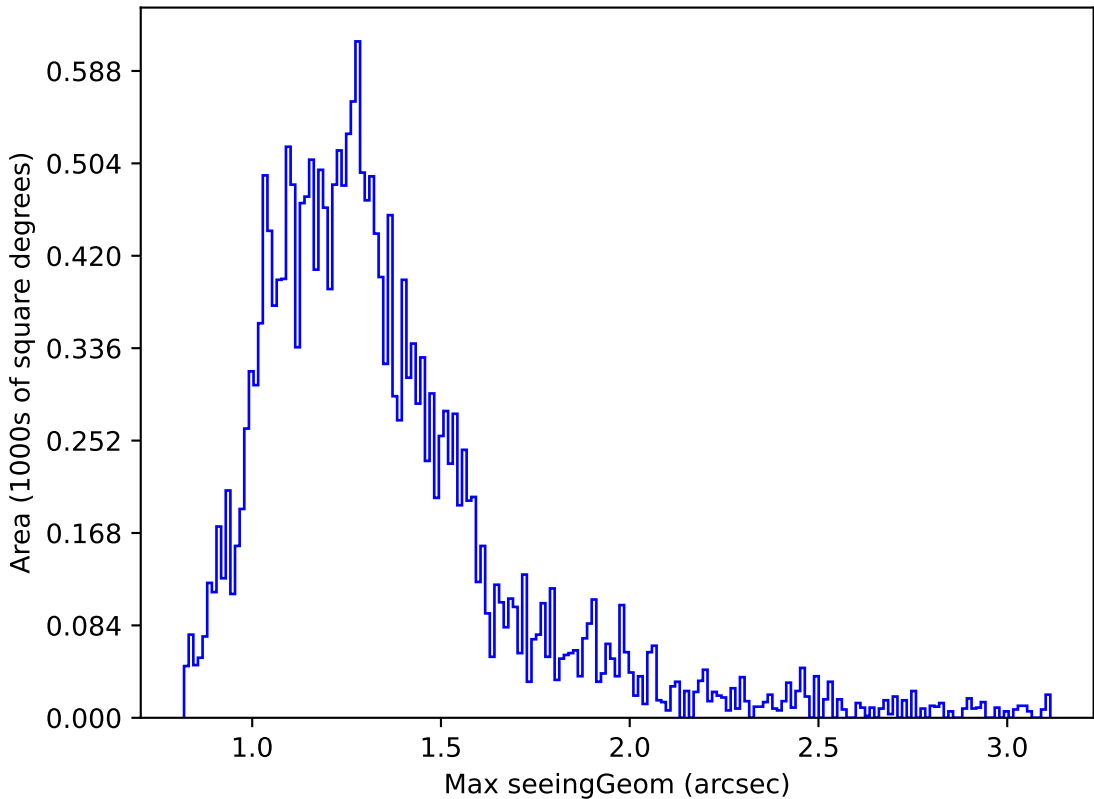
too_elab_r256_d2_gz_v3.4_10yrs Yr 1 u band: Max seeingGeom
