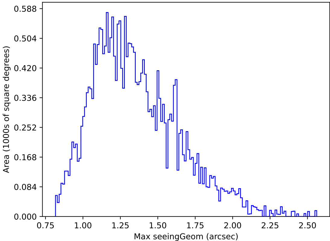
too_elab_r256_d2_gz_v3.4_10yrs Yr 1 r band: Max seeingGeom
