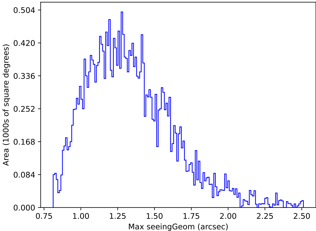
too_elab_r256_d2_gz_v3.4_10yrs Yr 1 g band: Max seeingGeom
