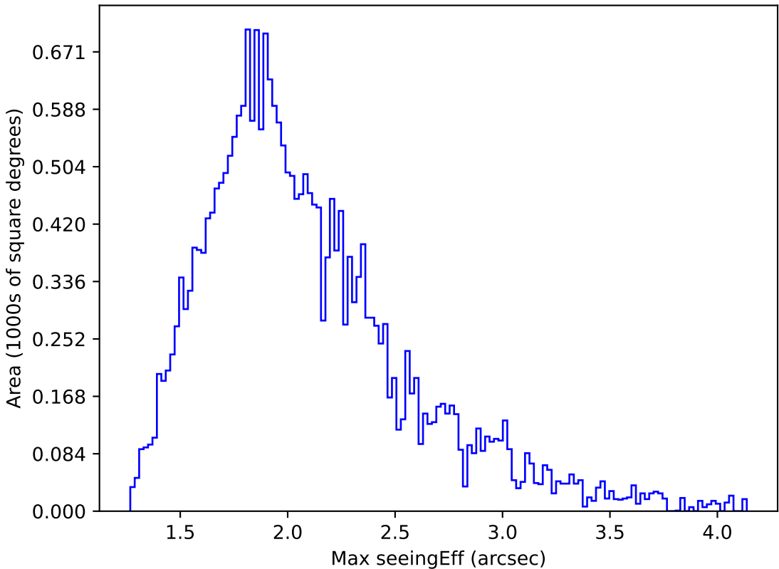
too_elab_r256_d2_gz_v3.4_10yrs Yr 1 all bands: Max seeingEff
