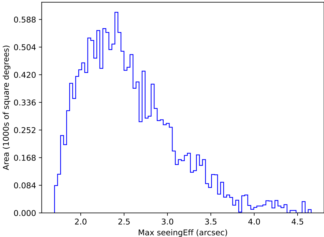
too_elab_r256_d2_gz_v3.4_10yrs WFD z band: Max seeingEff
