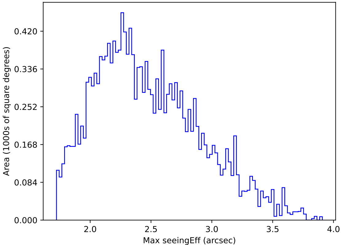
too_elab_r256_d2_gz_v3.4_10yrs WFD u band: Max seeingEff
