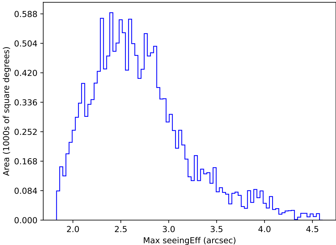
too_elab_r256_d2_gz_v3.4_10yrs WFD r band: Max seeingEff
