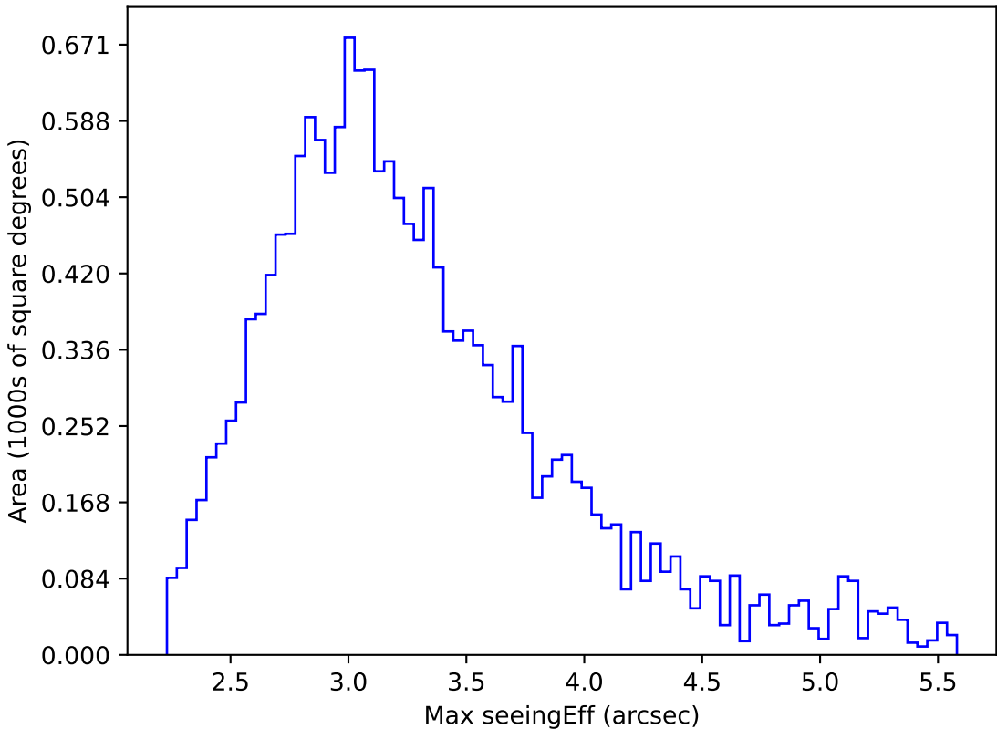
too_elab_r256_d2_gz_v3.4_10yrs WFD all bands: Max seeingEff
