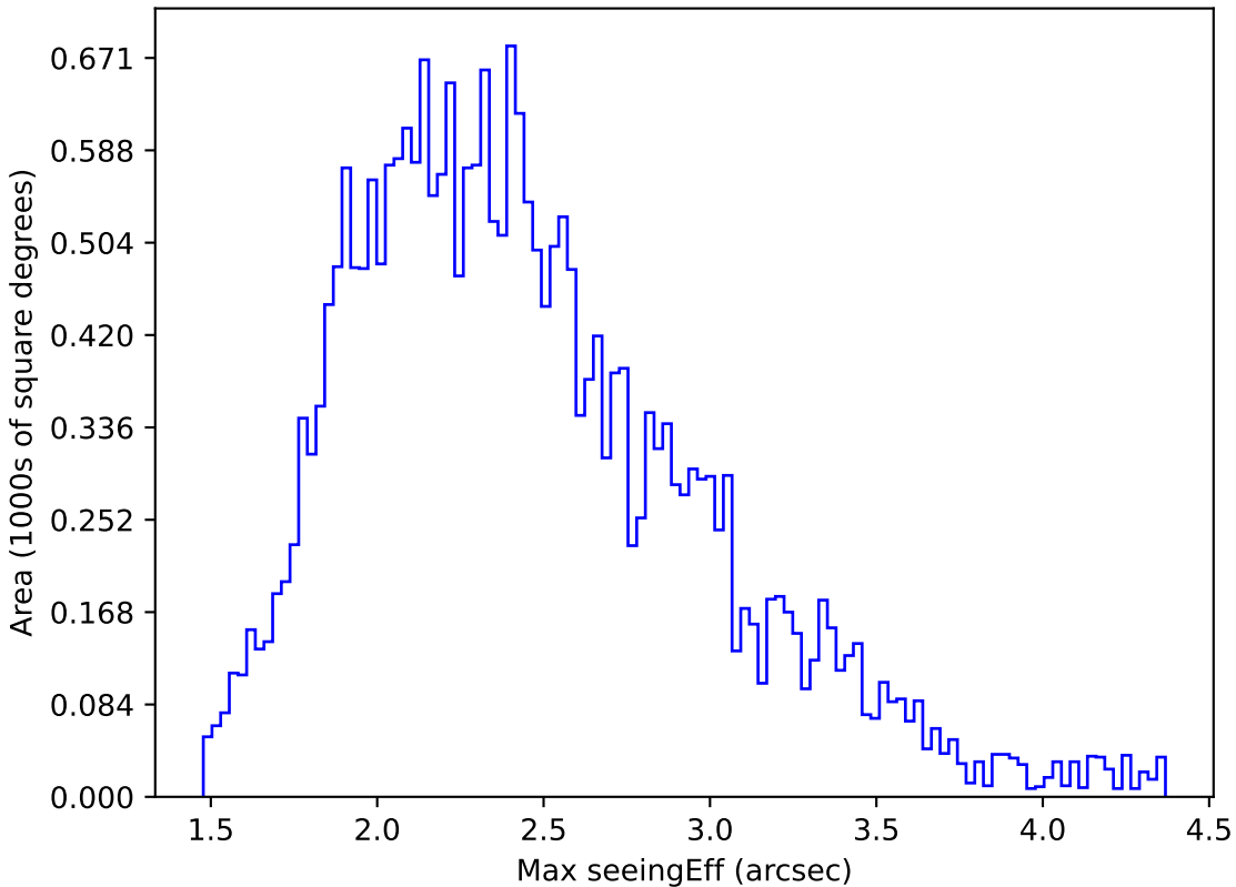
too_elab_r256_d2_gz_v3.4_10yrs All sky z band: Max seeingEff
