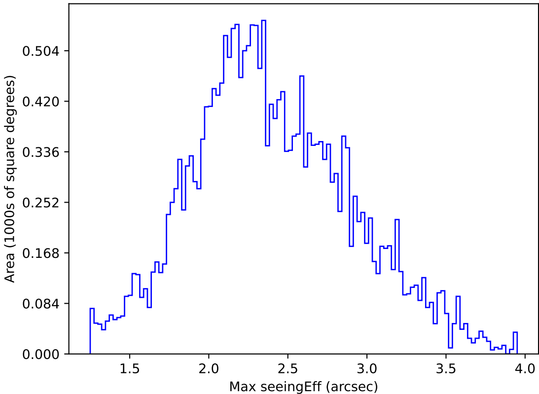
too_elab_r256_d2_gz_v3.4_10yrs All sky u band: Max seeingEff
