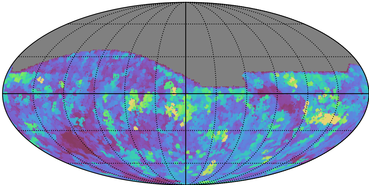
too_elab_r256_d2_gz_v3.4_10yrs All sky r band: Max seeingEff
