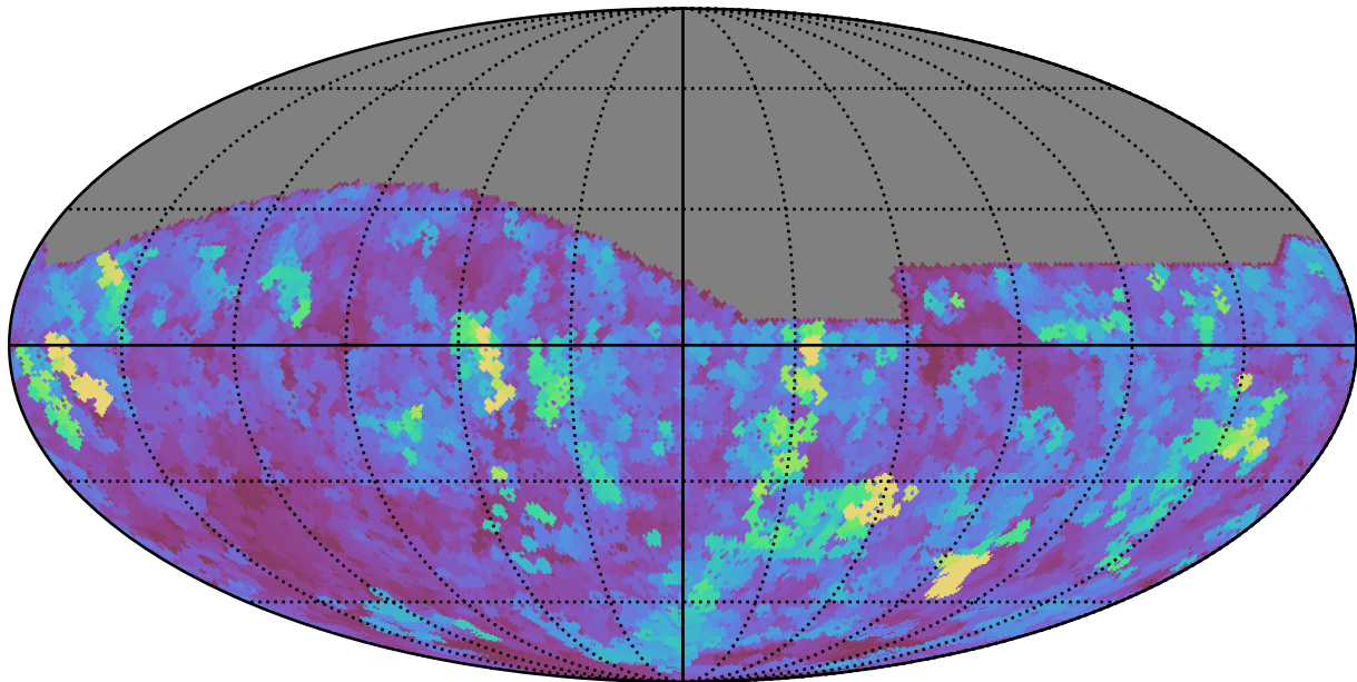
too_elab_r256_d2_gz_v3.4_10yrs All sky i band: Max seeingEff
