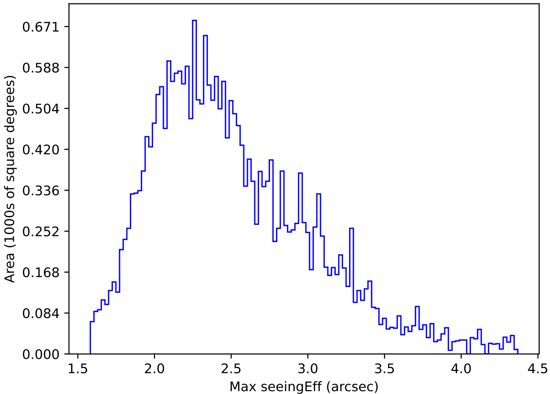
too_elab_r256_d2_gz_v3.4_10yrs All sky g band: Max seeingEff
