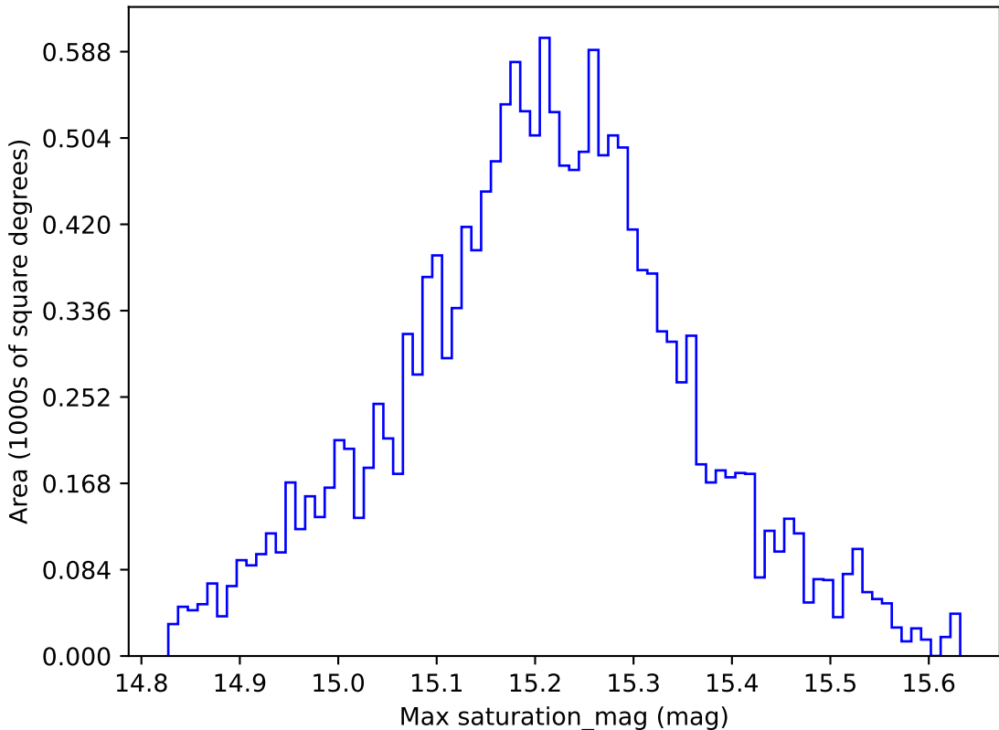
too_elab_r256_d2_gz_v3.4_10yrs WFD z band: Max saturation_mag
