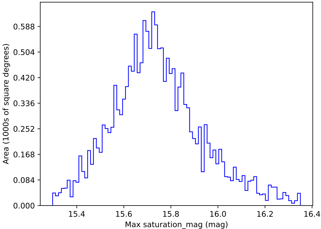
too_elab_r256_d2_gz_v3.4_10yrs WFD g band: Max saturation_mag
