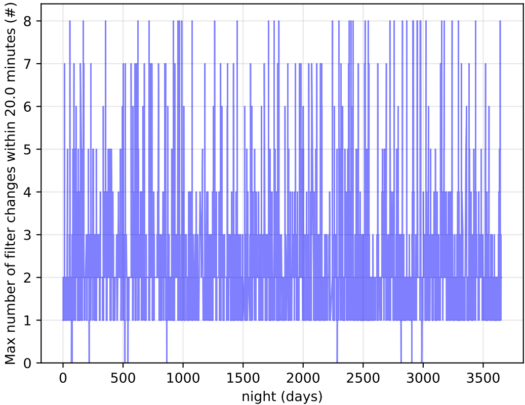
too_elab_r256_d2_gz_v3.4_10yrs Per Night: Max number of filter changes within 20.0 minutes
