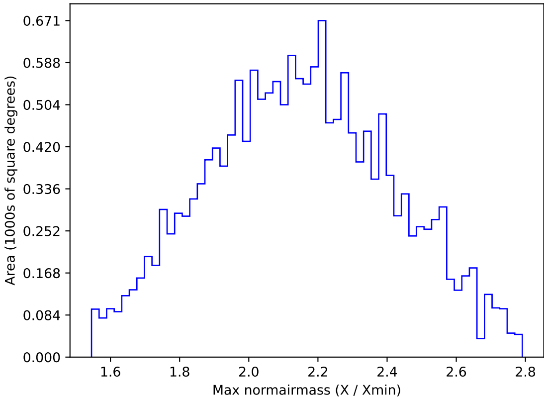
too_elab_r256_d2_gz_v3.4_10yrs WFD y band: Max normairmass
