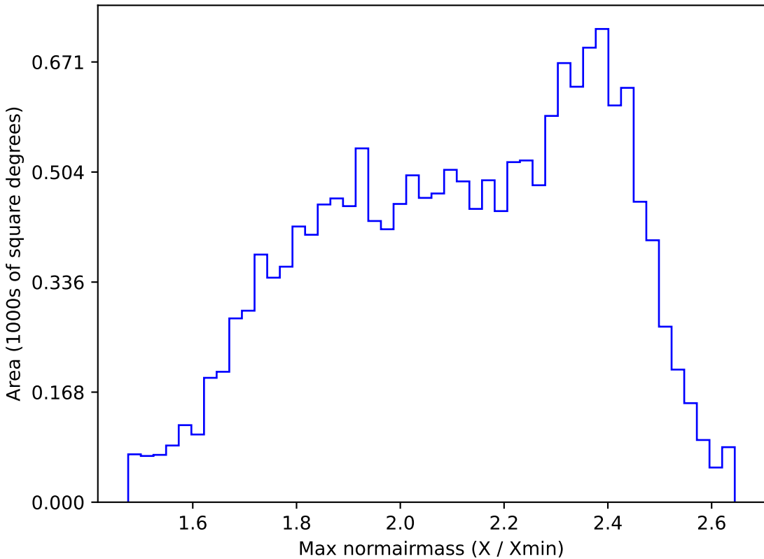
too_elab_r256_d2_gz_v3.4_10yrs WFD r band: Max normairmass
