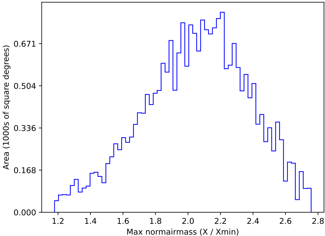
too_elab_r256_d2_gz_v3.4_10yrs All sky y band: Max normairmass
