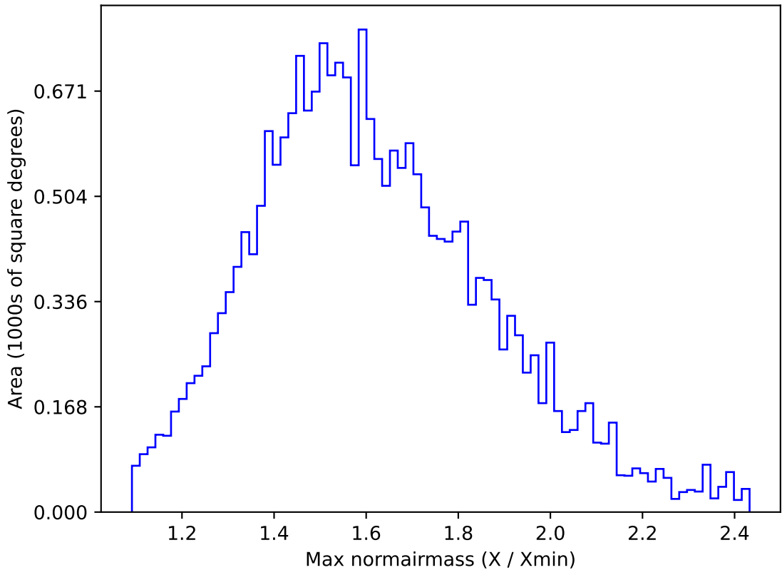
too_elab_r256_d2_gz_v3.4_10yrs All sky u band: Max normairmass
