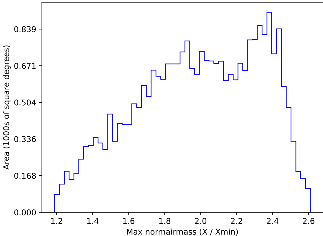
too_elab_r256_d2_gz_v3.4_10yrs All sky r band: Max normairmass
