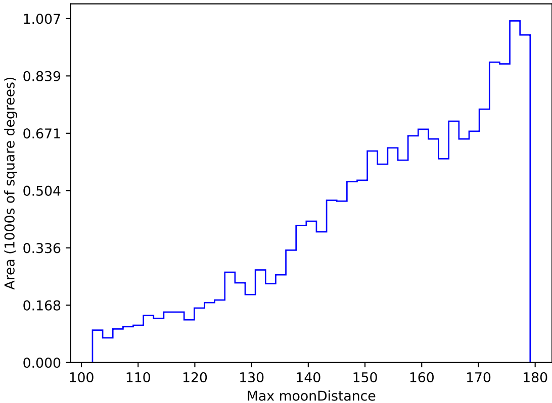
too_elab_r256_d2_gz_v3.4_10yrs WFD u band: Max moonDistance
