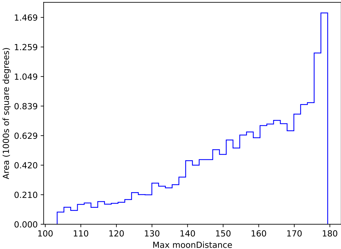
too_elab_r256_d2_gz_v3.4_10yrs WFD r band: Max moonDistance
