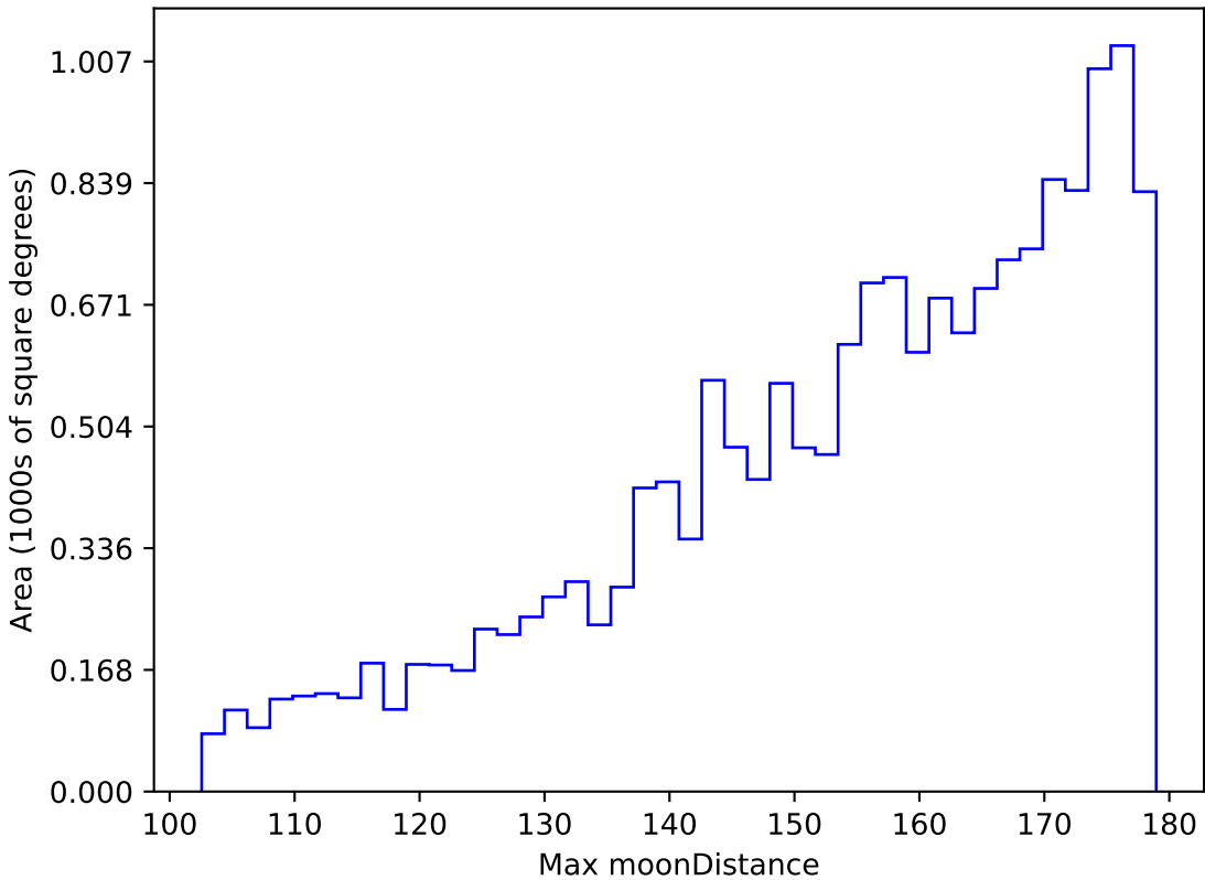
too_elab_r256_d2_gz_v3.4_10yrs WFD g band: Max moonDistance
