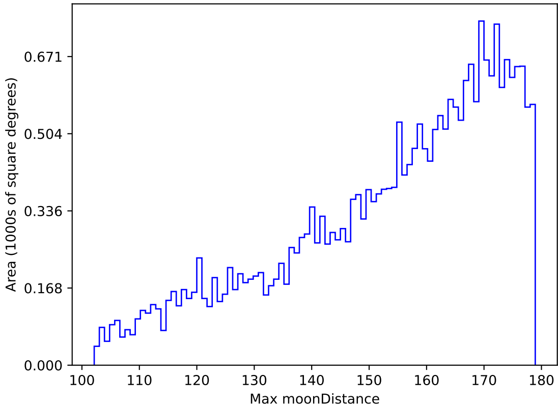
too_elab_r256_d2_gz_v3.4_10yrs All sky z band: Max moonDistance
