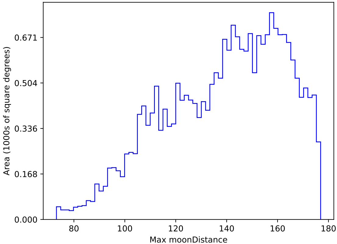
too_elab_r256_d2_gz_v3.4_10yrs All sky y band: Max moonDistance
